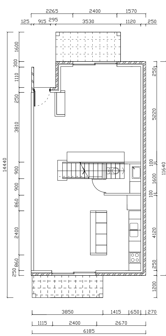
Ground Floor
